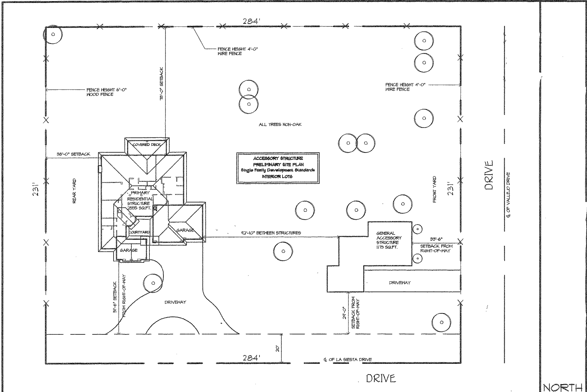
PROPOSED SITE PLAN SCALE: 1" = 40'-0"
